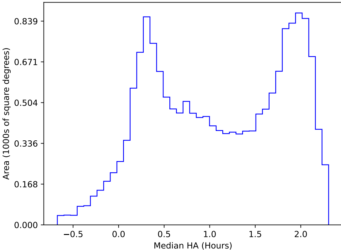
too_elab_r256_d3_griz_v3.4_10yrs WFD i band: Median HA
