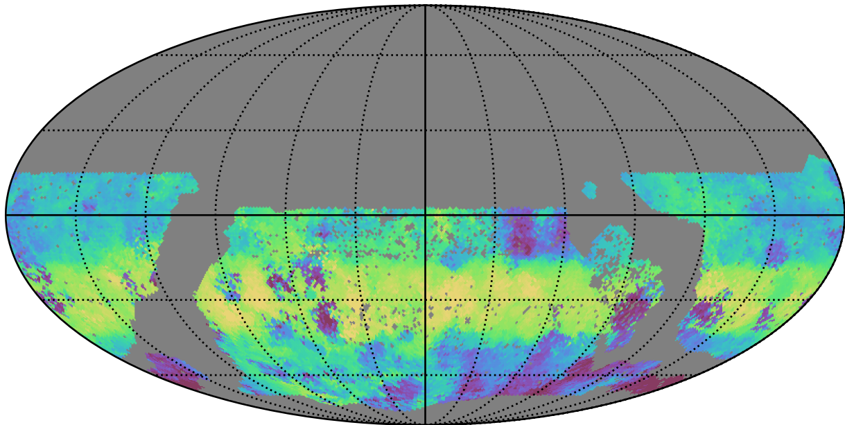
too_elab_r256_d3_griz_v3.4_10yrs WFD g band: Median HA
