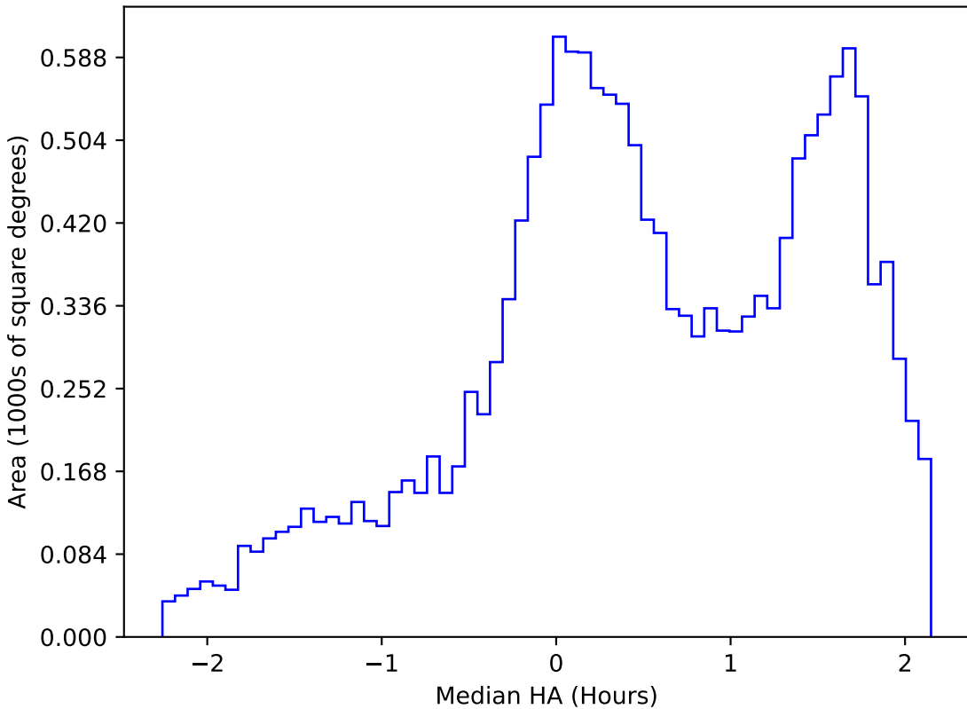
too_elab_r256_d3_griz_v3.4_10yrs WFD g band: Median HA
