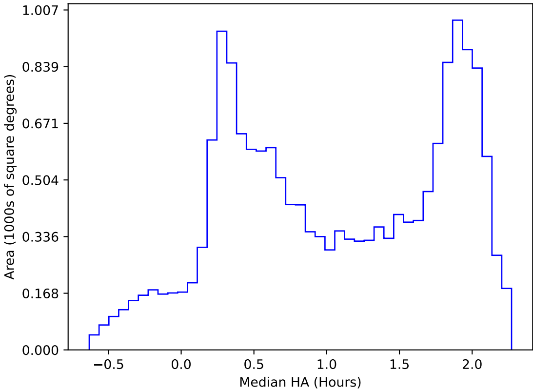
too_elab_r256_d3_griz_v3.4_10yrs WFD all bands: Median HA
