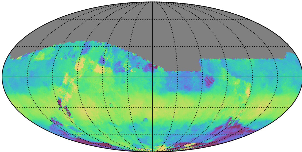
too_elab_r256_d3_griz_v3.4_10yrs All sky z band: Median HA
