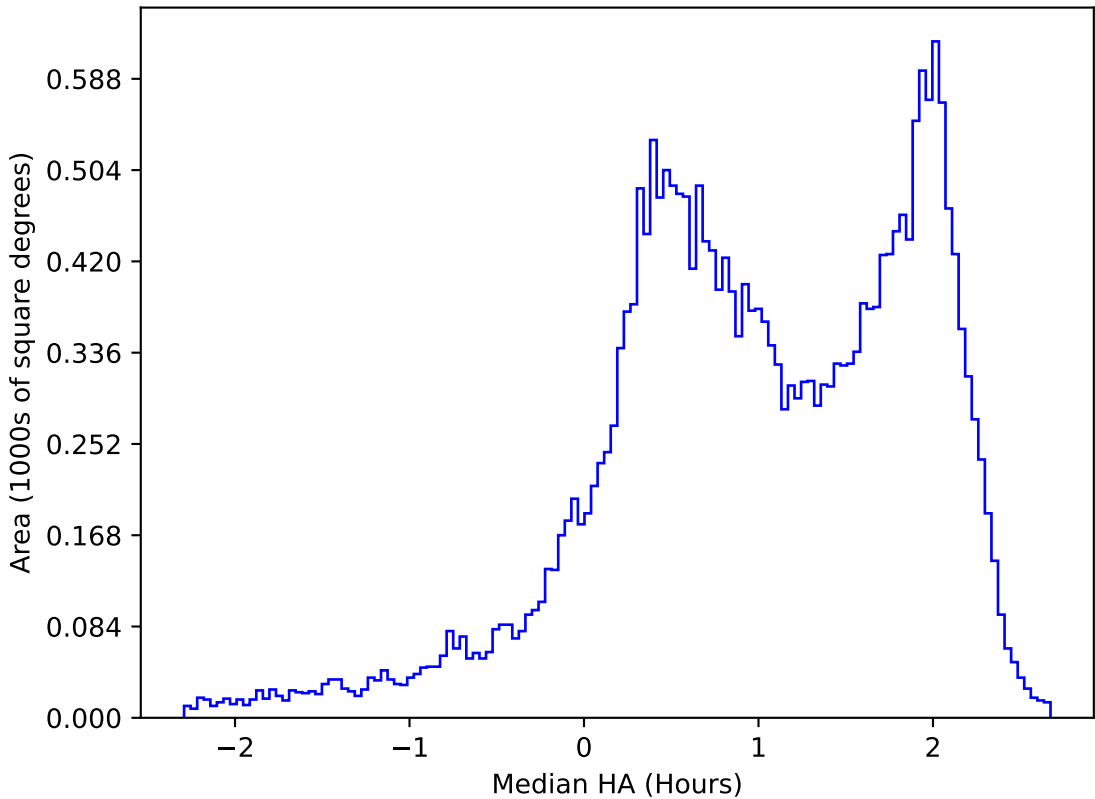
too_elab_r256_d3_griz_v3.4_10yrs All sky z band: Median HA
