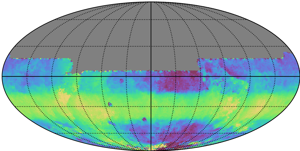
too_elab_r256_d3_griz_v3.4_10yrs All sky y band: Median HA
