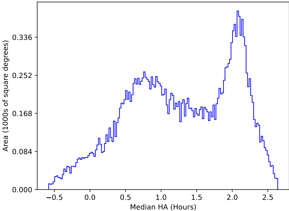
too_elab_r256_d3_griz_v3.4_10yrs All sky y band: Median HA
