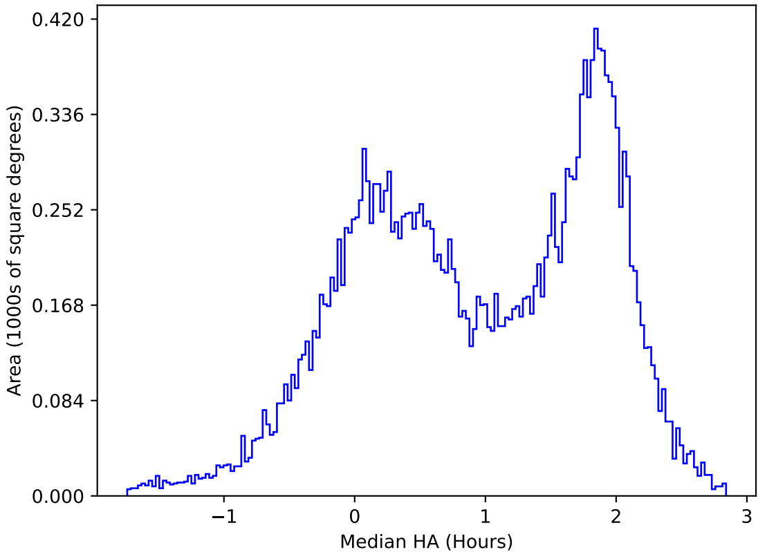
too_elab_r256_d3_griz_v3.4_10yrs All sky u band: Median HA
