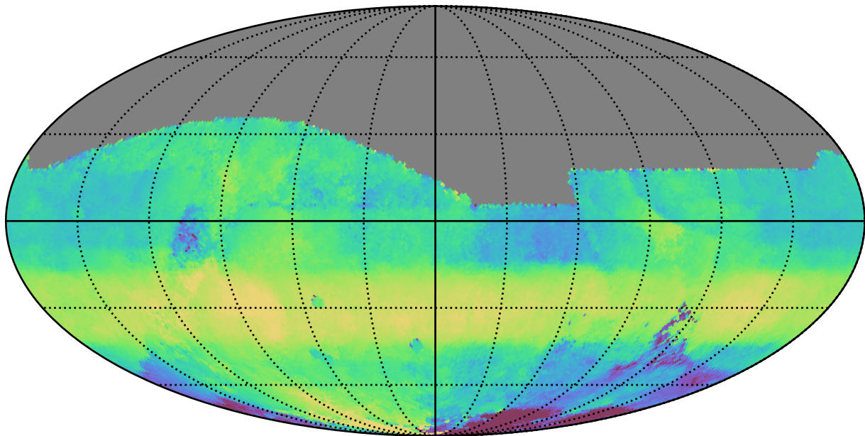
too_elab_r256_d3_griz_v3.4_10yrs All sky r band: Median HA
