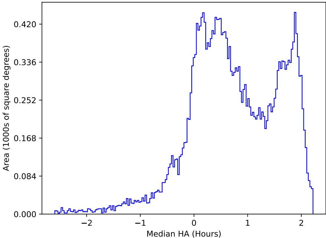
too_elab_r256_d3_griz_v3.4_10yrs All sky r band: Median HA
