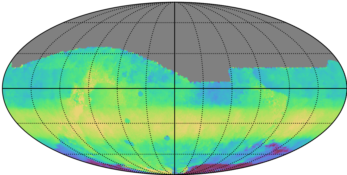
too_elab_r256_d3_griz_v3.4_10yrs All sky i band: Median HA
