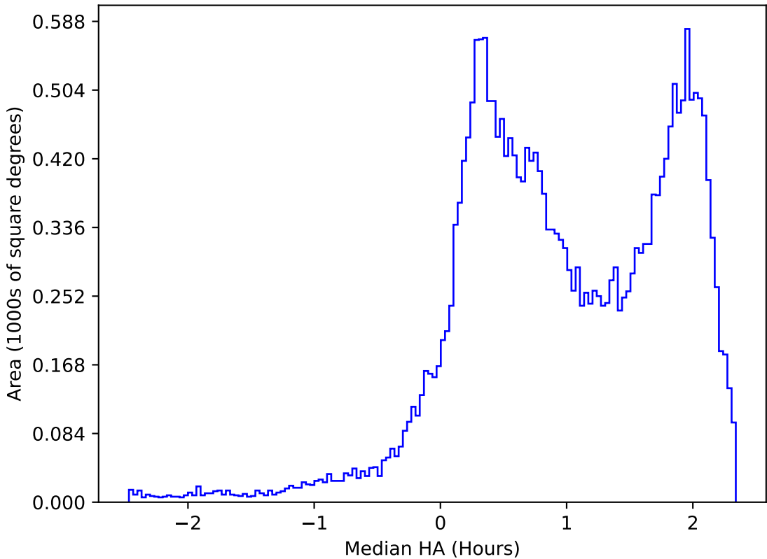
too_elab_r256_d3_griz_v3.4_10yrs All sky i band: Median HA
