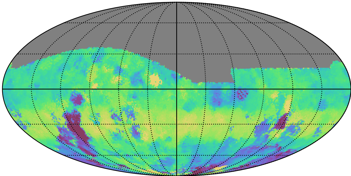
too_elab_r256_d3_griz_v3.4_10yrs All sky g band: Median HA
