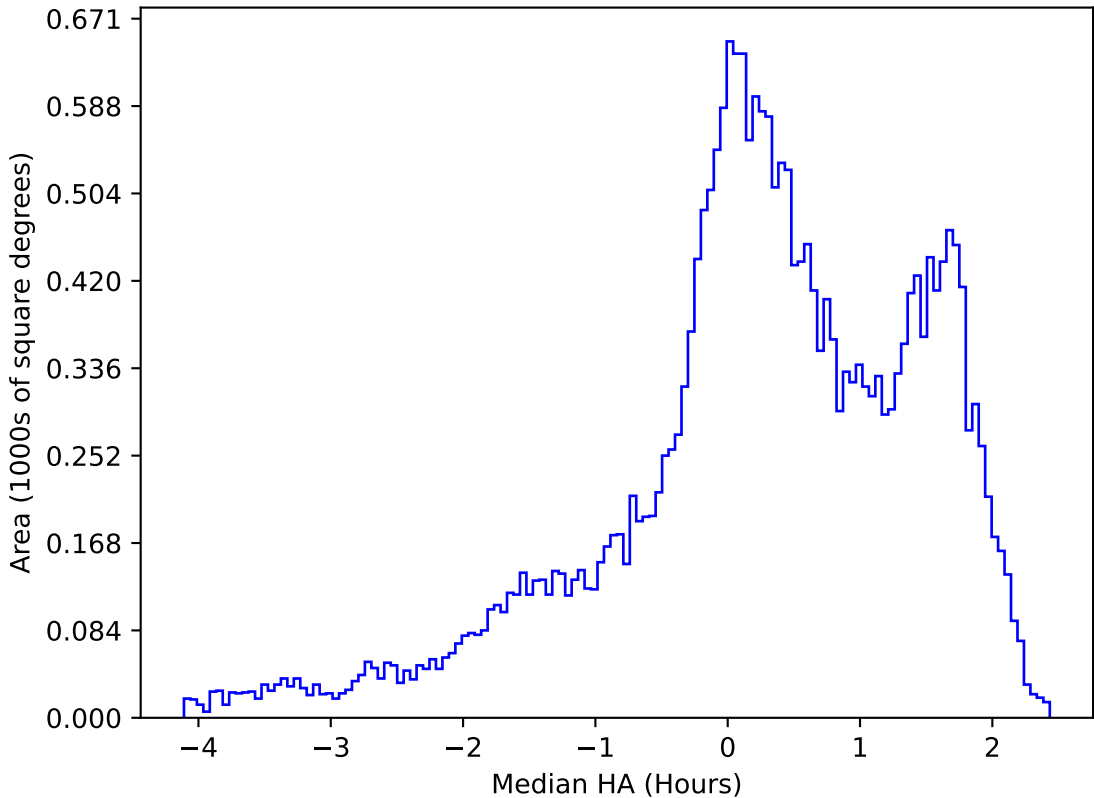
too_elab_r256_d3_griz_v3.4_10yrs All sky g band: Median HA
