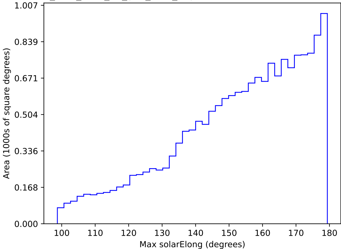
too_elab_r256_d3_griz_v3.4_10yrs WFD z band: Max solarElong
