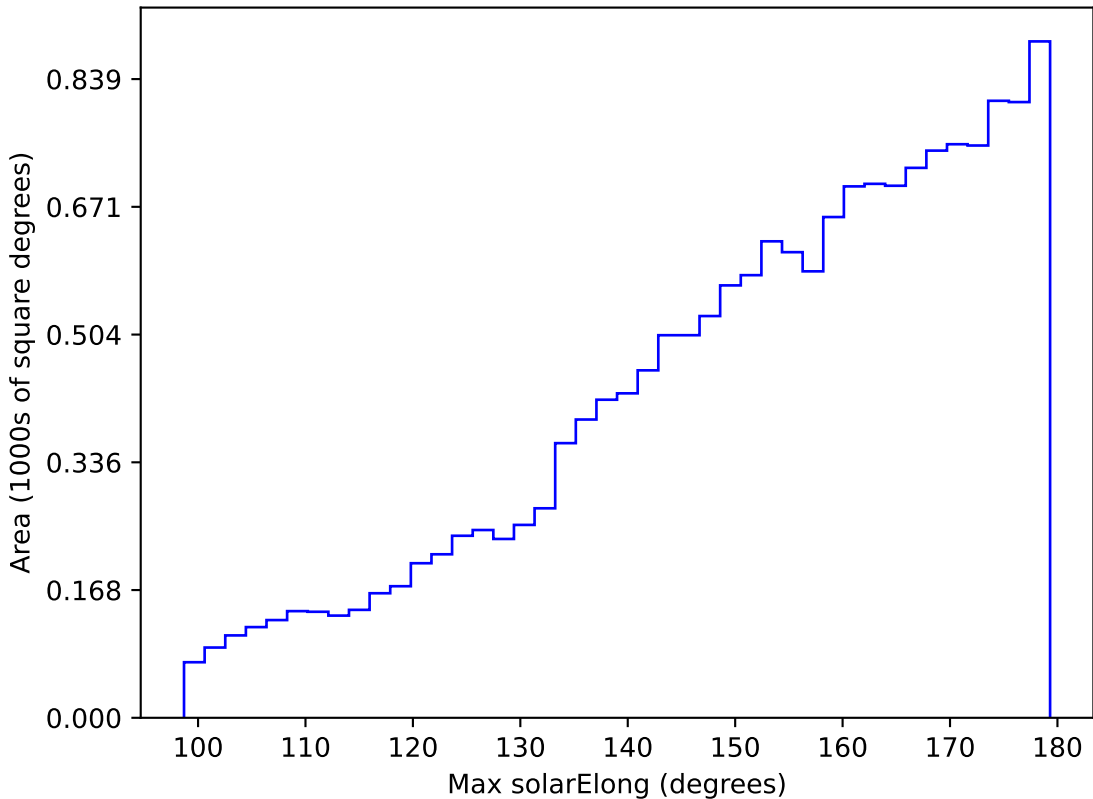
too_elab_r256_d3_griz_v3.4_10yrs WFD y band: Max solarElong
