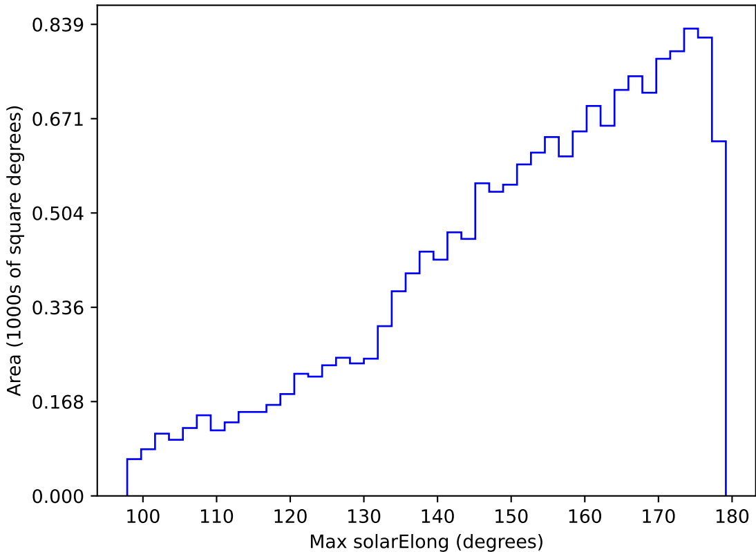
too_elab_r256_d3_griz_v3.4_10yrs WFD u band: Max solarElong
