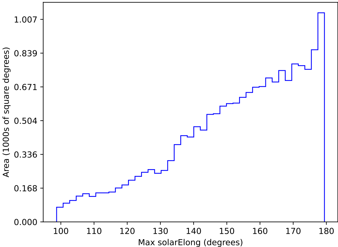
too_elab_r256_d3_griz_v3.4_10yrs WFD i band: Max solarElong
