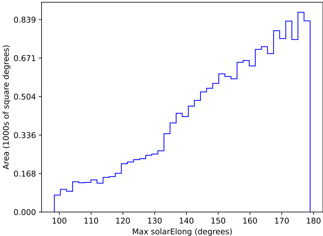
too_elab_r256_d3_griz_v3.4_10yrs WFD g band: Max solarElong
