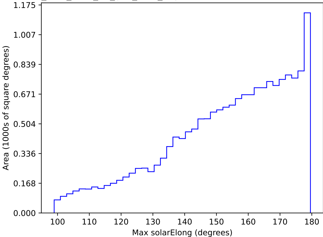
too_elab_r256_d3_griz_v3.4_10yrs WFD all bands: Max solarElong
