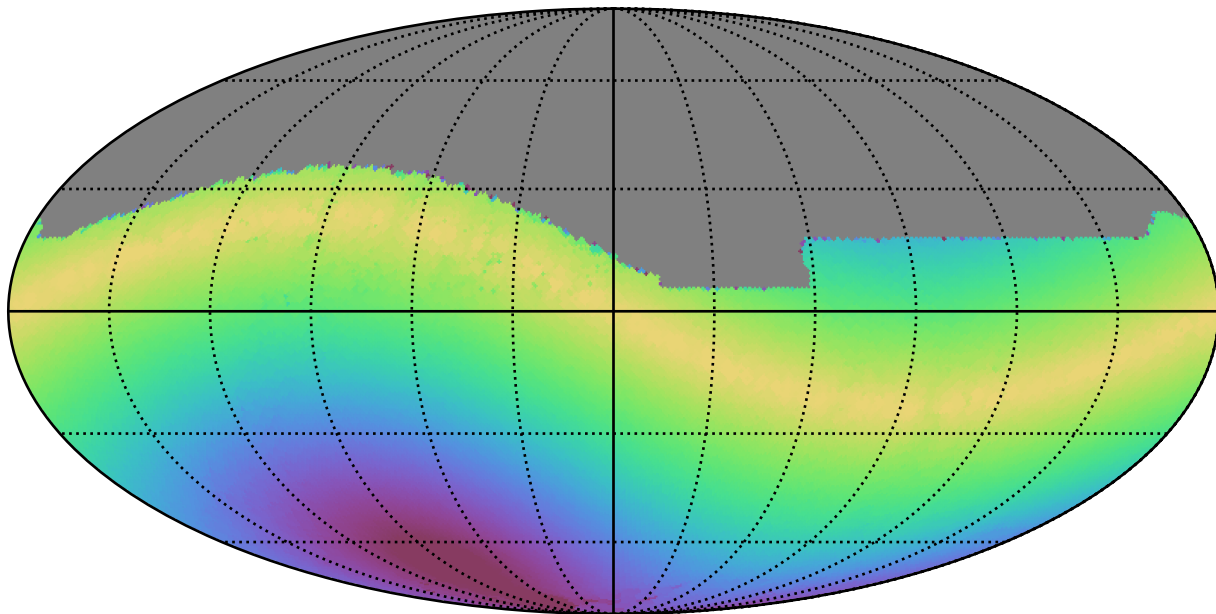
too_elab_r256_d3_griz_v3.4_10yrs All sky z band: Max solarElong
