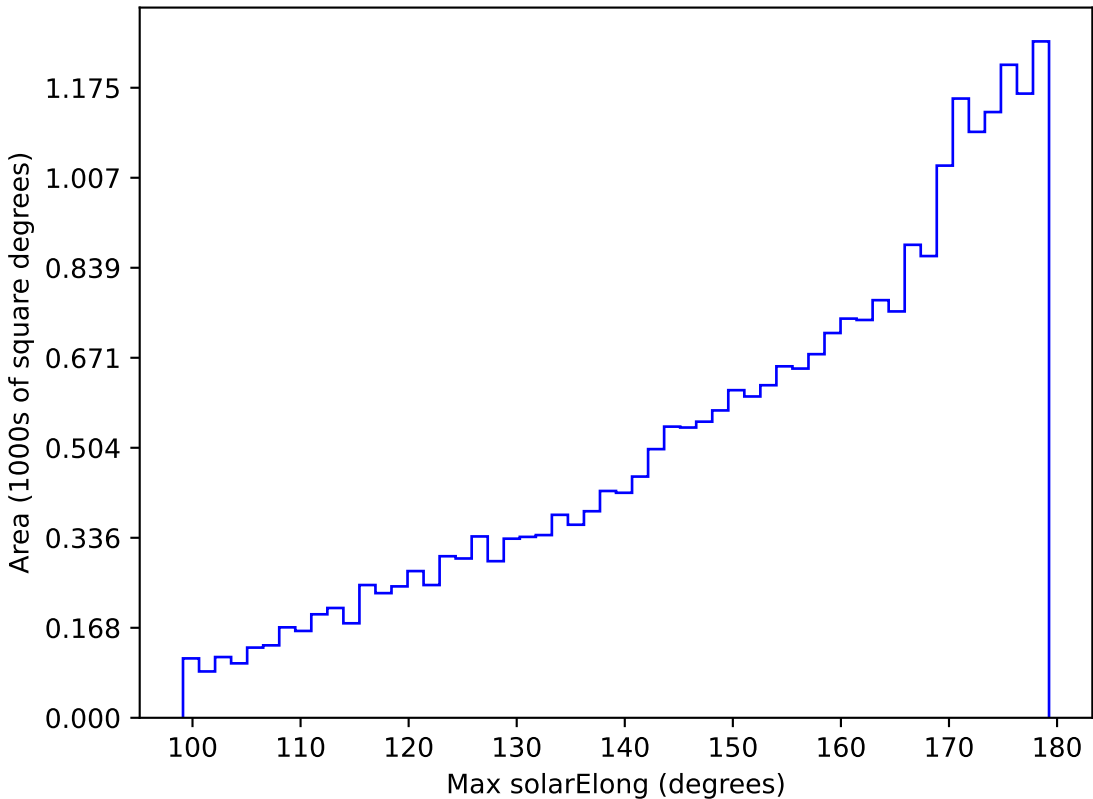
too_elab_r256_d3_griz_v3.4_10yrs All sky z band: Max solarElong
