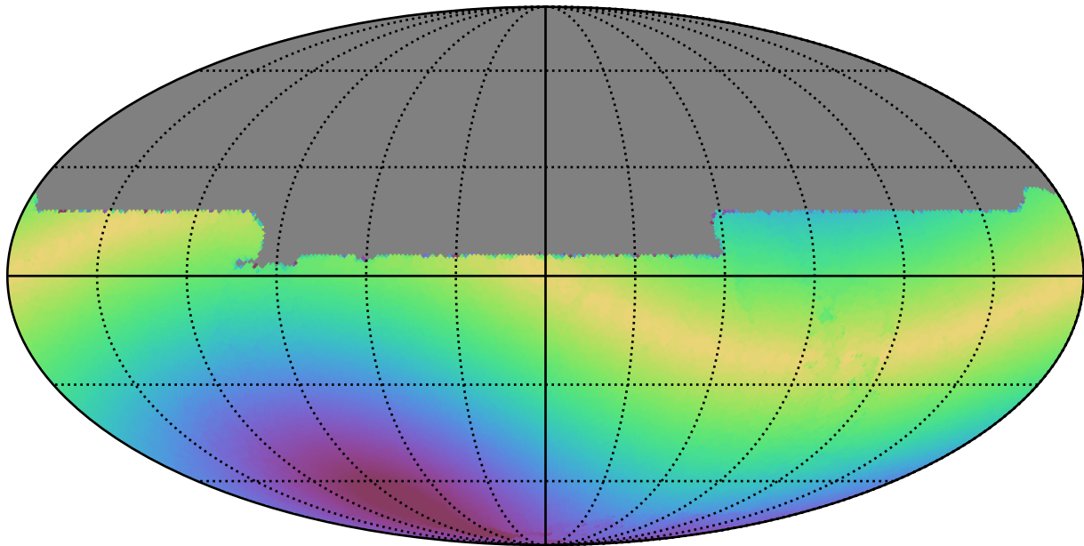
too_elab_r256_d3_griz_v3.4_10yrs All sky y band: Max solarElong
