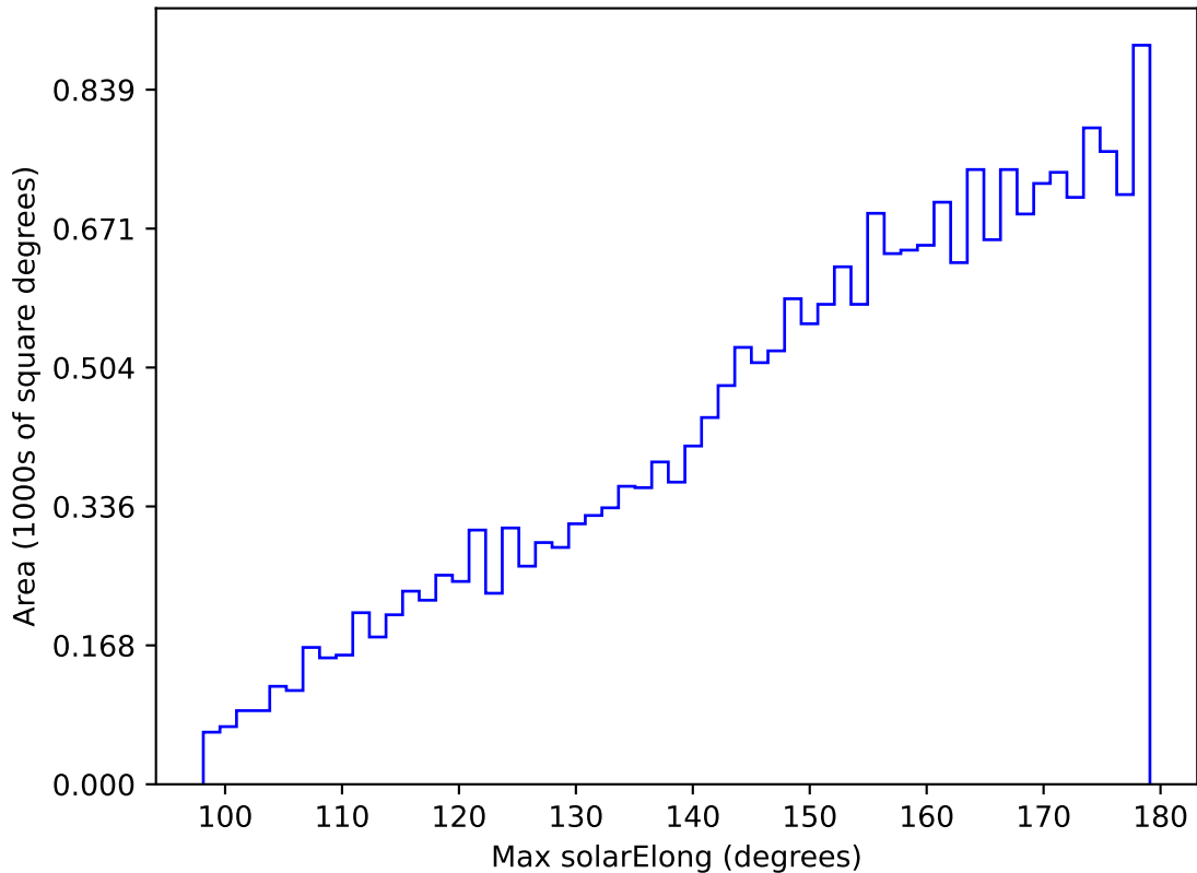
too_elab_r256_d3_griz_v3.4_10yrs All sky y band: Max solarElong
