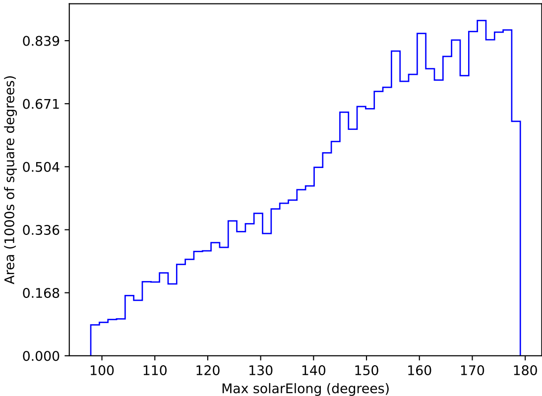
too_elab_r256_d3_griz_v3.4_10yrs All sky u band: Max solarElong
