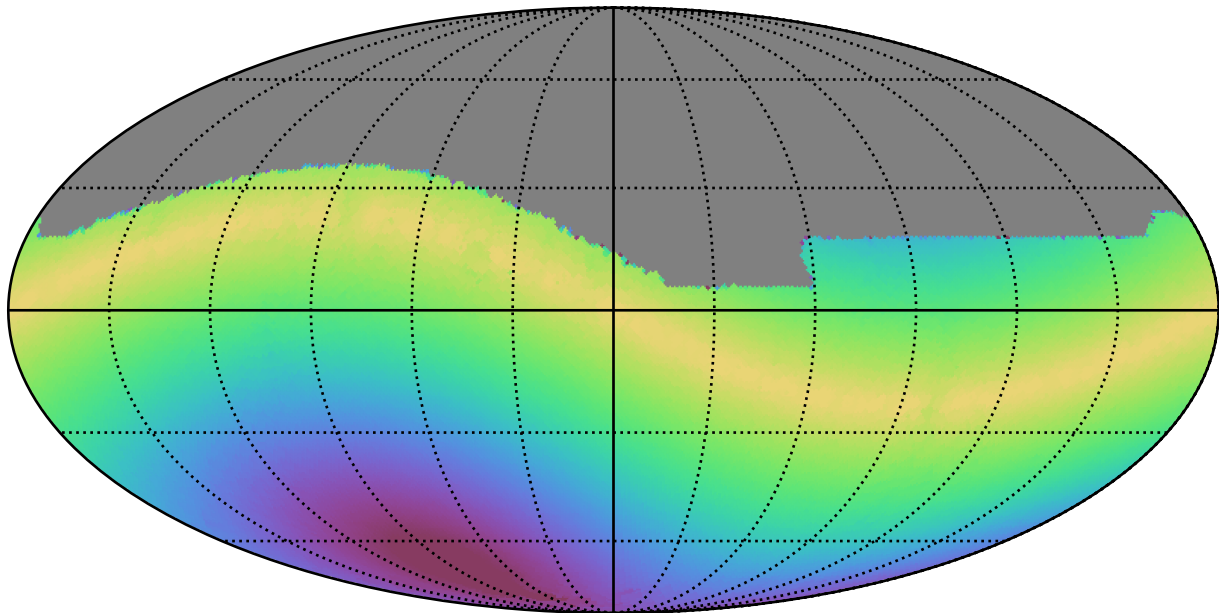
too_elab_r256_d3_griz_v3.4_10yrs All sky r band: Max solarElong
