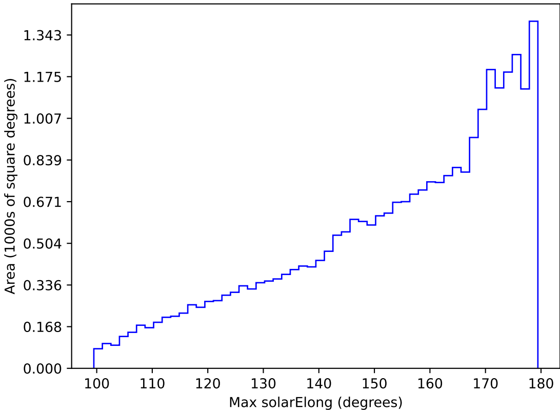
too_elab_r256_d3_griz_v3.4_10yrs All sky r band: Max solarElong
