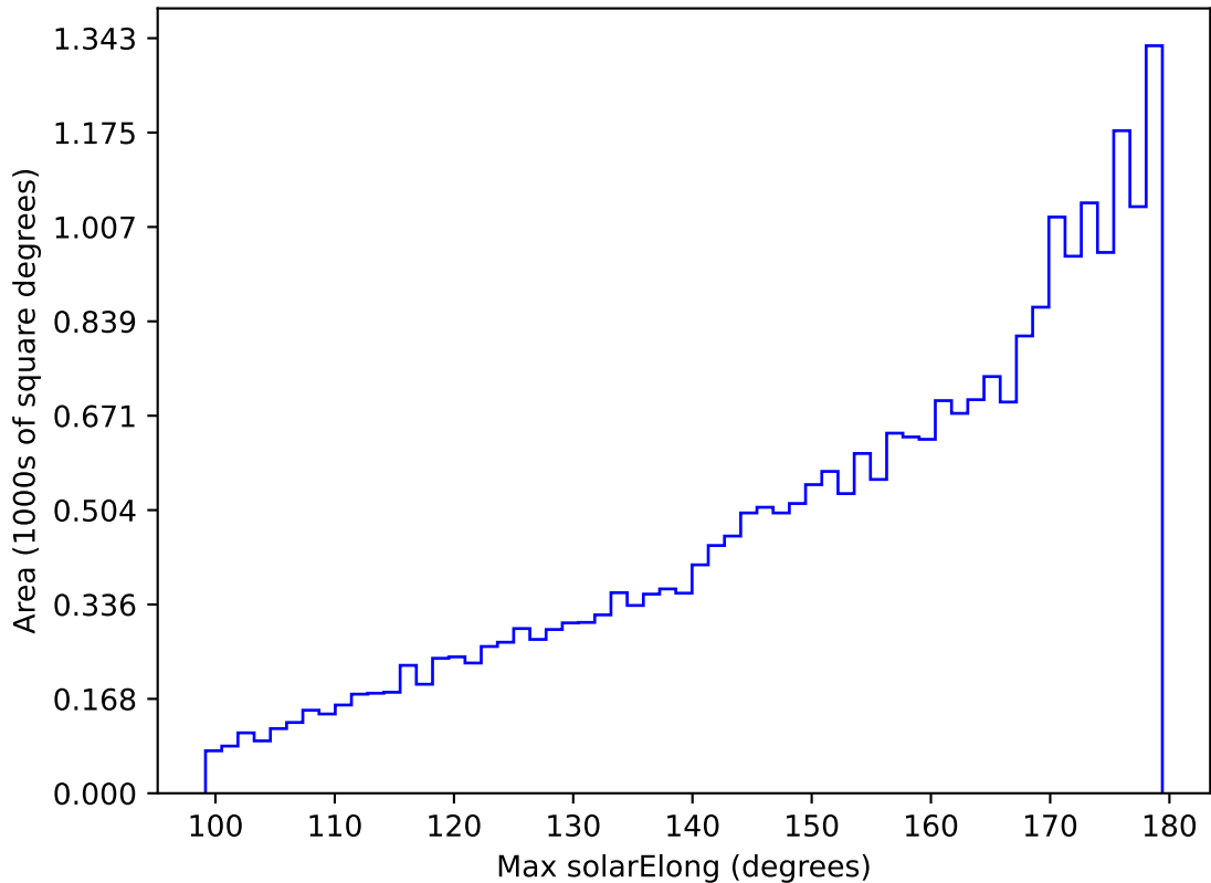
too_elab_r256_d3_griz_v3.4_10yrs All sky i band: Max solarElong
