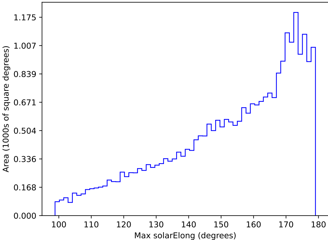
too_elab_r256_d3_griz_v3.4_10yrs All sky g band: Max solarElong
