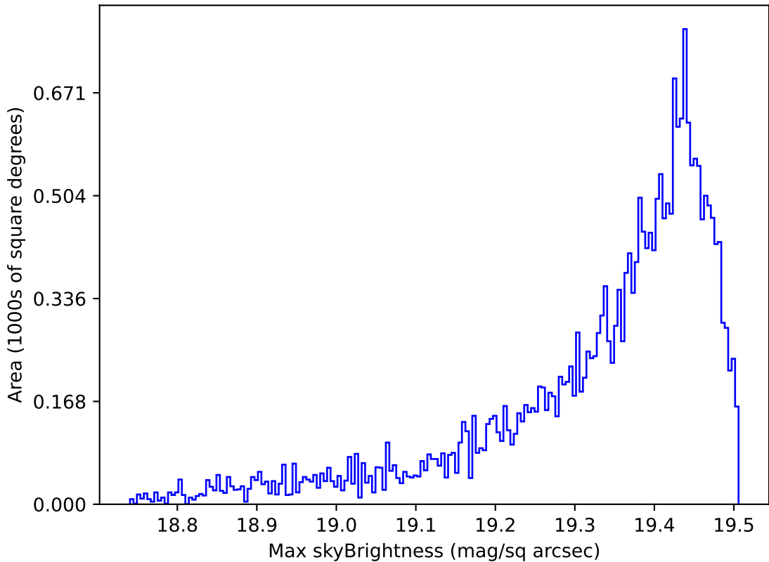
too_elab_r256_d3_griz_v3.4_10yrs Yr 1 z band: Max skyBrightness
