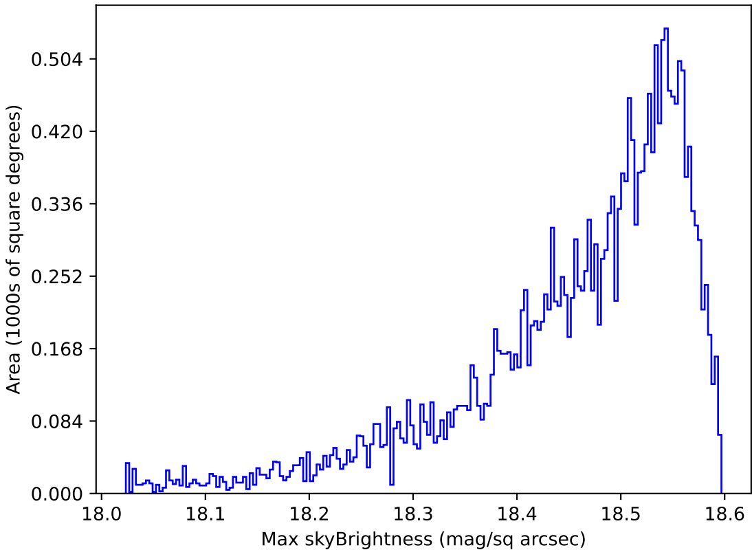
too_elab_r256_d3_griz_v3.4_10yrs Yr 1 y band: Max skyBrightness
