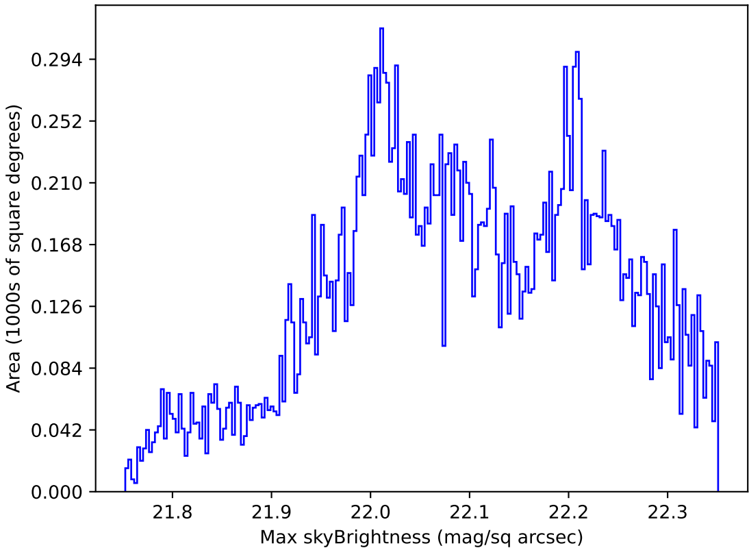
too_elab_r256_d3_griz_v3.4_10yrs Yr 1 g band: Max skyBrightness
