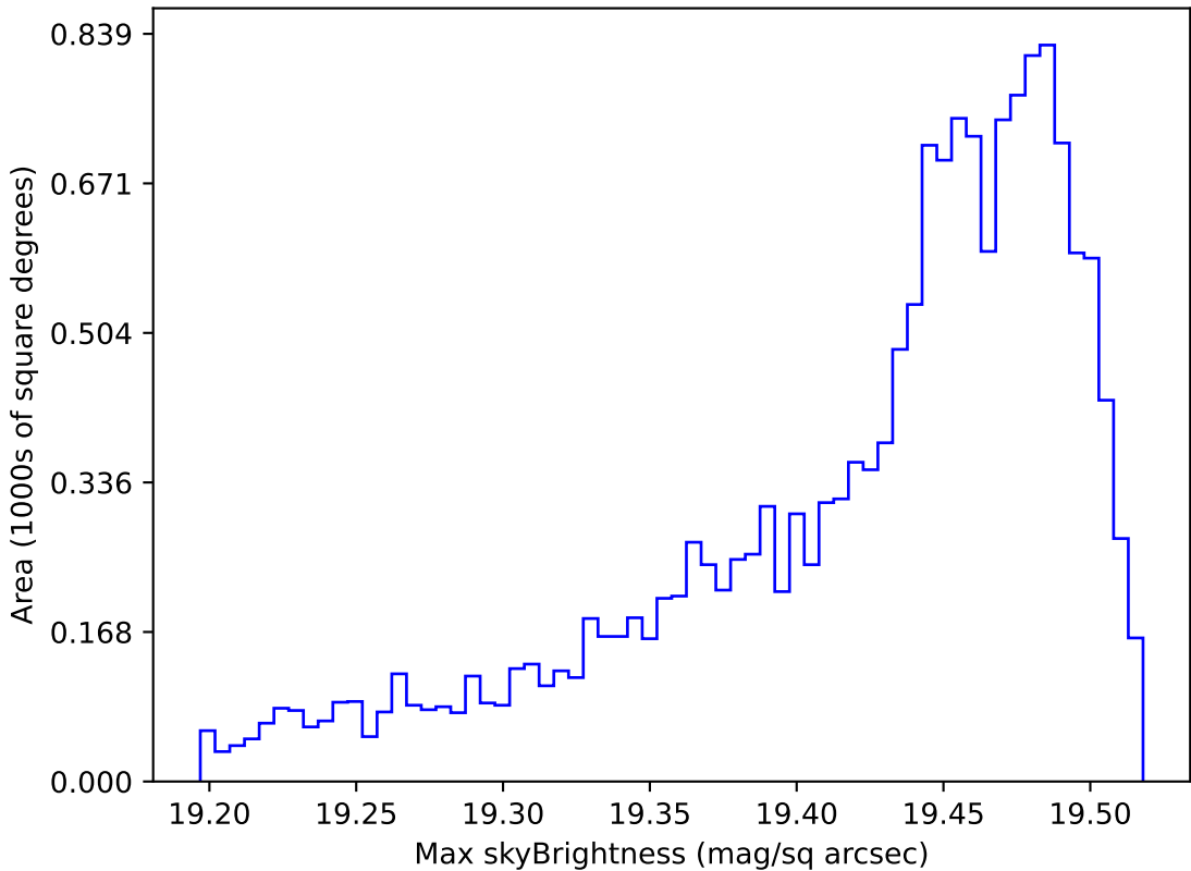
too_elab_r256_d3_griz_v3.4_10yrs WFD z band: Max skyBrightness
