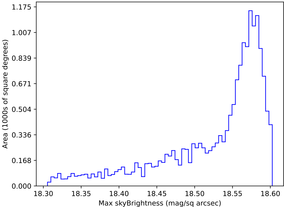
too_elab_r256_d3_griz_v3.4_10yrs WFD y band: Max skyBrightness
