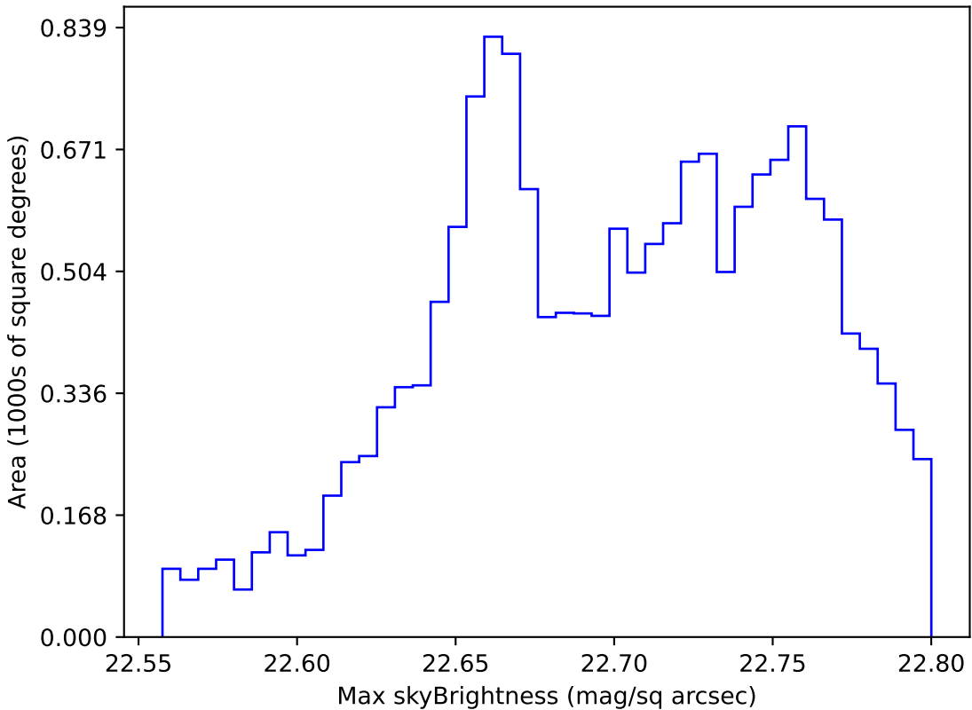
too_elab_r256_d3_griz_v3.4_10yrs WFD u band: Max skyBrightness
