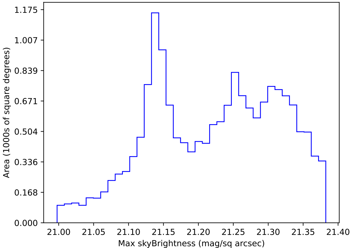
too_elab_r256_d3_griz_v3.4_10yrs WFD r band: Max skyBrightness
