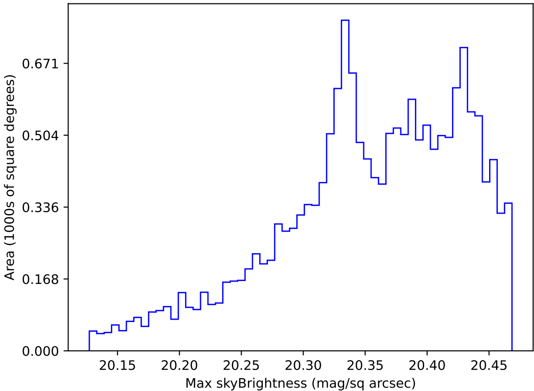
too_elab_r256_d3_griz_v3.4_10yrs WFD i band: Max skyBrightness
