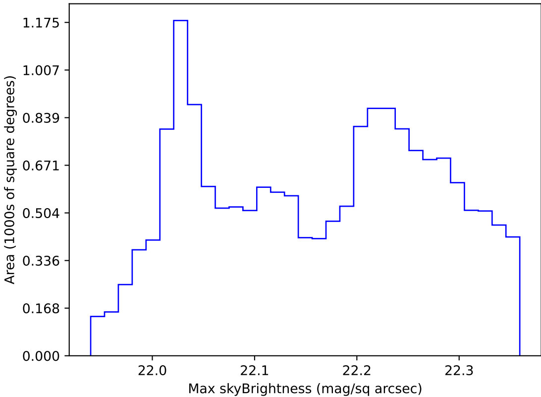
too_elab_r256_d3_griz_v3.4_10yrs WFD g band: Max skyBrightness
