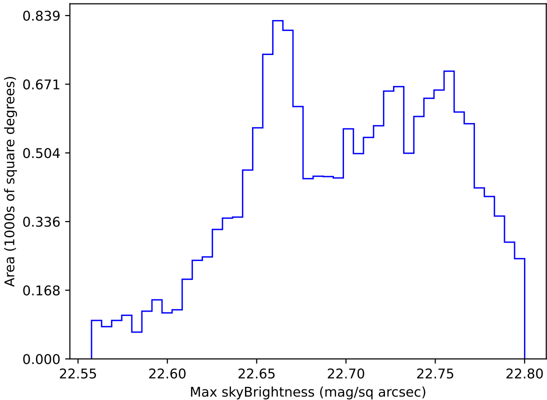
too_elab_r256_d3_griz_v3.4_10yrs WFD all bands: Max skyBrightness
