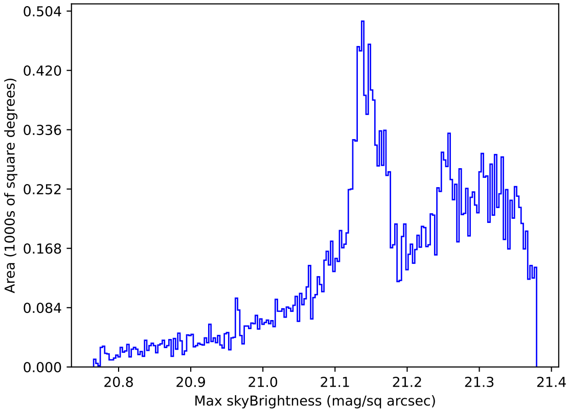
too_elab_r256_d3_griz_v3.4_10yrs All sky r band: Max skyBrightness
