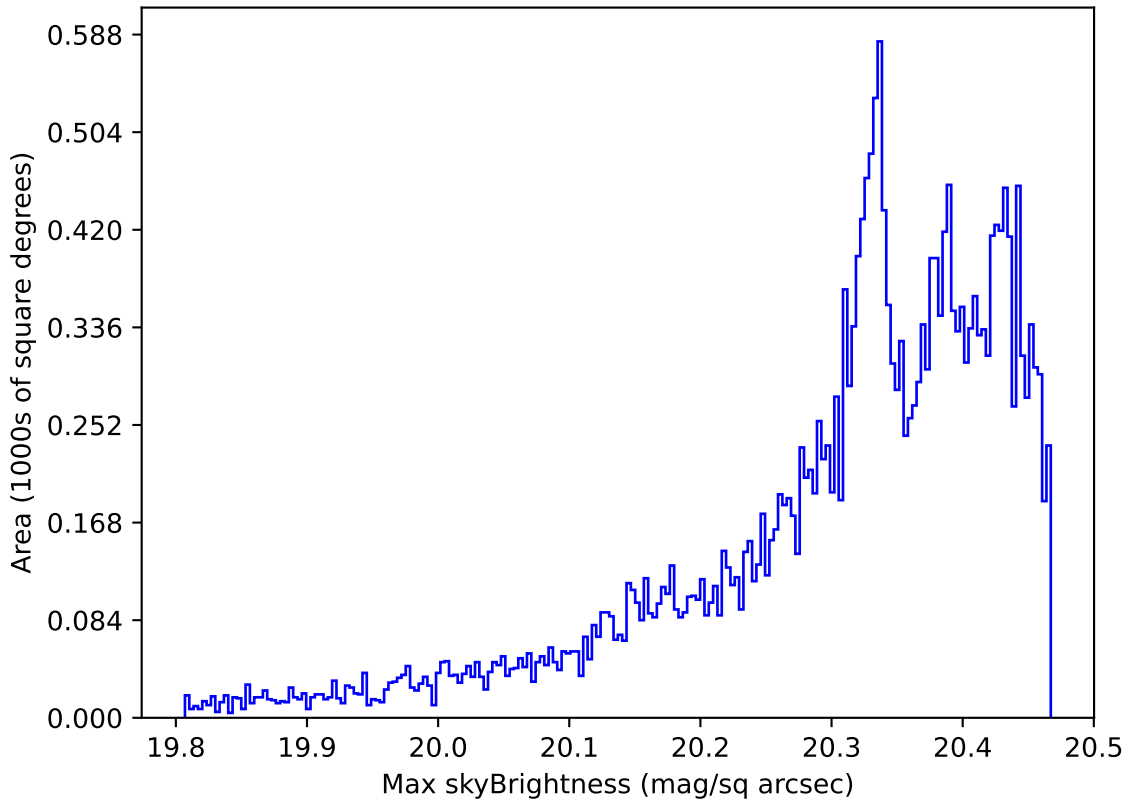
too_elab_r256_d3_griz_v3.4_10yrs All sky i band: Max skyBrightness
