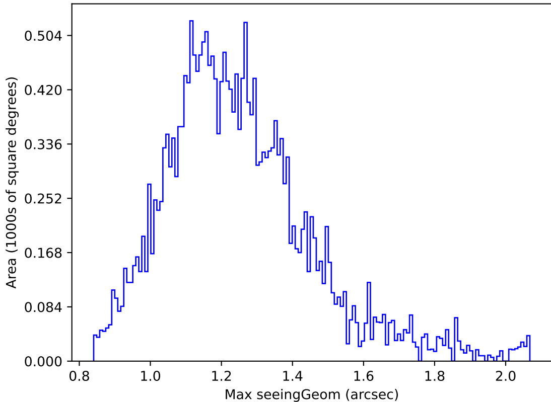
too_elab_r256_d3_griz_v3.4_10yrs Yr 1 y band: Max seeingGeom
