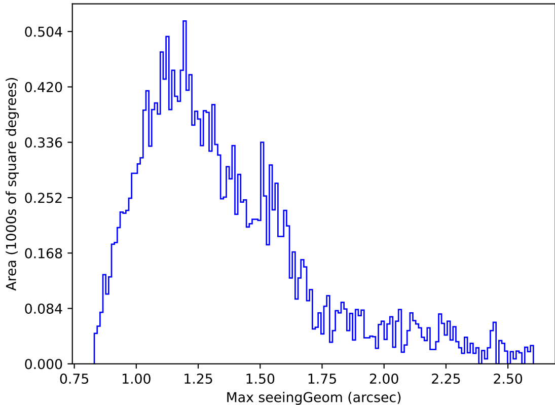
too_elab_r256_d3_griz_v3.4_10yrs Yr 1 u band: Max seeingGeom
