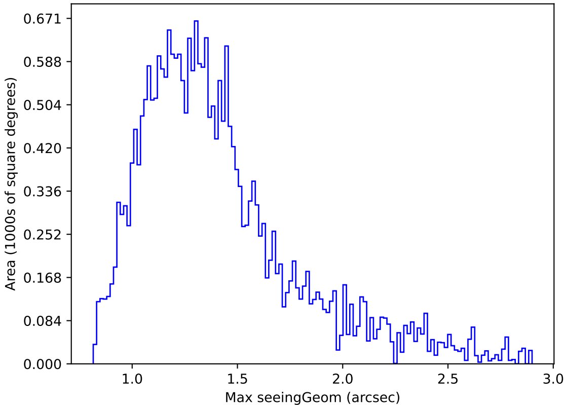
too_elab_r256_d3_griz_v3.4_10yrs Yr 1 i band: Max seeingGeom
