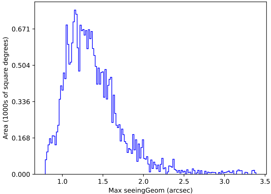
too_elab_r256_d3_griz_v3.4_10yrs Yr 1 g band: Max seeingGeom
