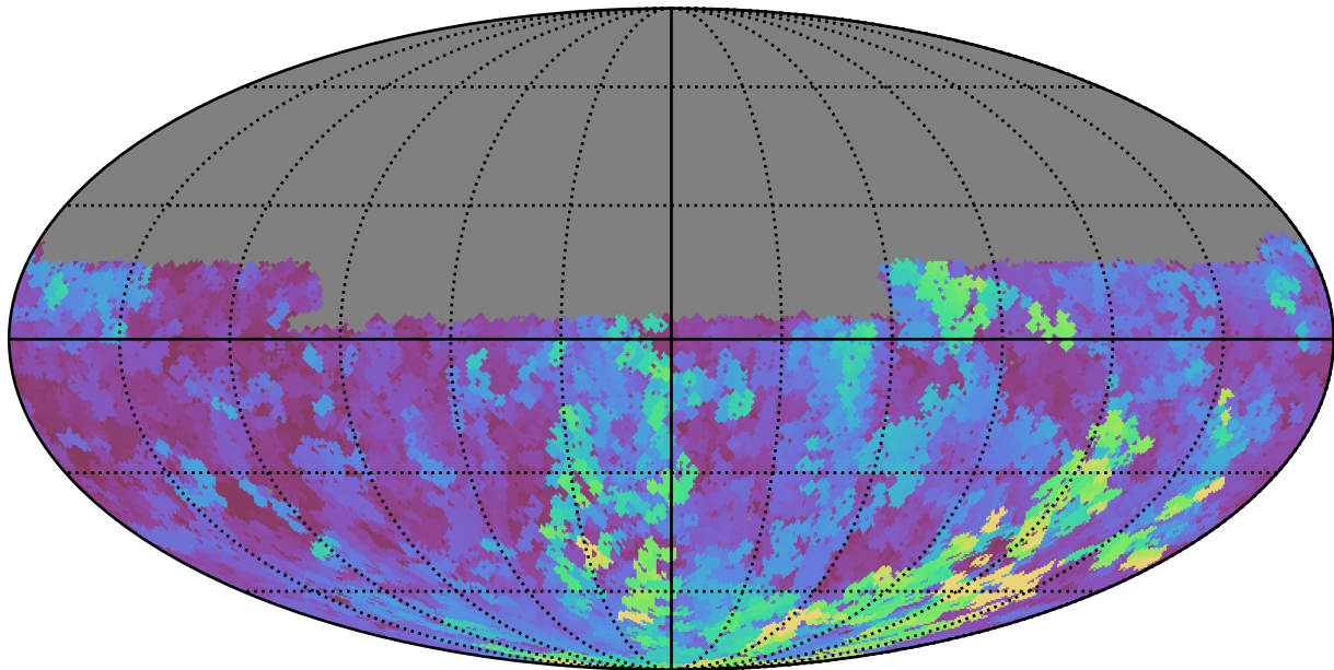
too_elab_r256_d3_griz_v3.4_10yrs Yr 1 u band: Max seeingEff
