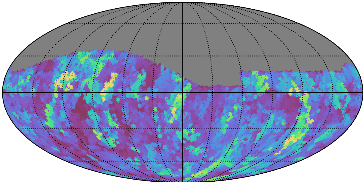
too_elab_r256_d3_griz_v3.4_10yrs Yr 1 r band: Max seeingEff
