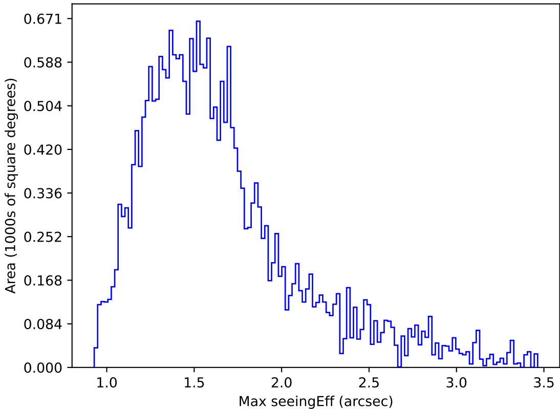
too_elab_r256_d3_griz_v3.4_10yrs Yr 1 i band: Max seeingEff
