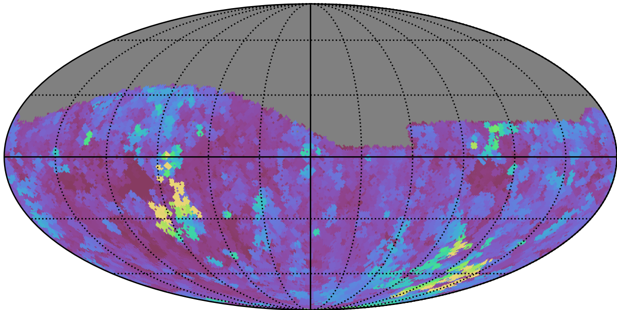
too_elab_r256_d3_griz_v3.4_10yrs Yr 1 g band: Max seeingEff
